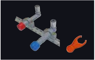
BUTE-1 Adjustable 1/2" BSP Male Wall Elbow BUTE1 - 1/2" BSP x 15mm x 70mm BUTE1EX - 1/2" BSP x 15mm x 100mm Includes telescopic steel brackets, test caps (hot & cold) and palm spanner.
