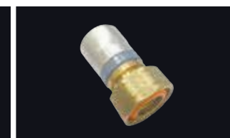
BRASS FEMALE SWIVELS F15BX - 1/2" BSP x 15mm F20BX - 3/4" BSP x 20mm F2015BX - 3/4" BSP x 15mm F2028B - 3/4" BSP x 28mm F28B - 1" BSP x 28mm
